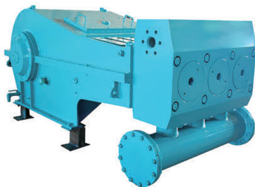
定向穿越泵 HDD (Trenchless) Pump
