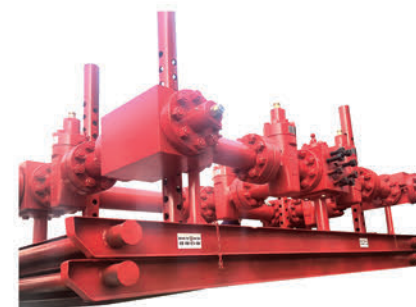
节流管汇 Choke Manifold
