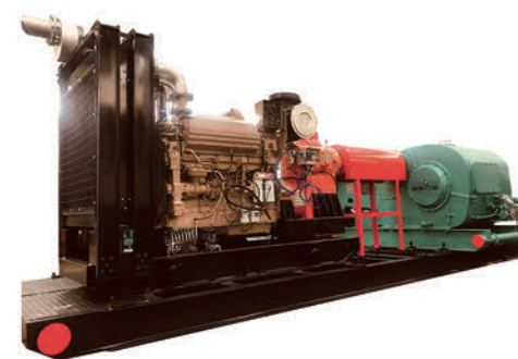
柴油机雷斯达变速箱泵组 Mud Pump c/w Cummings Engine +Reastar Gear
