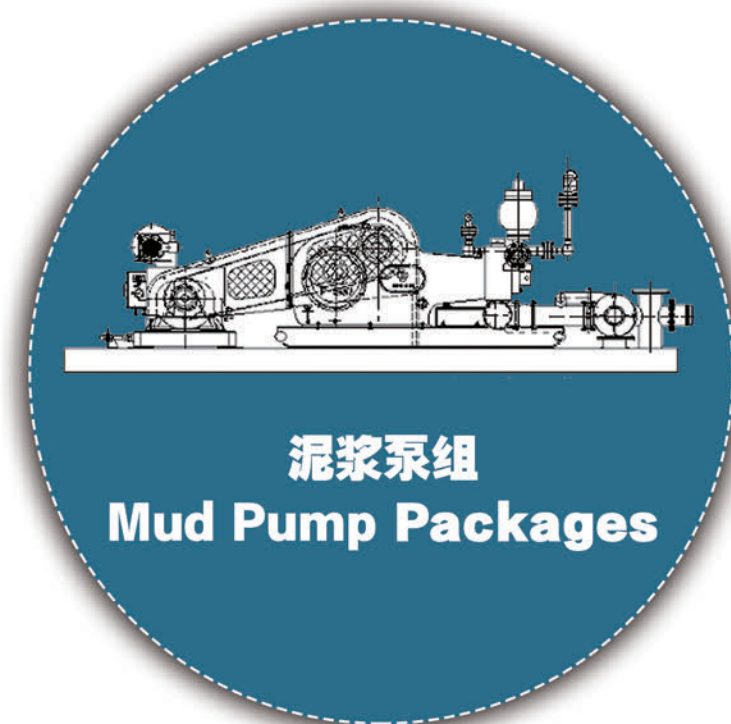
液力耦合器泵组 Mud Pump c/w diesel engine+hydraulic coupler
